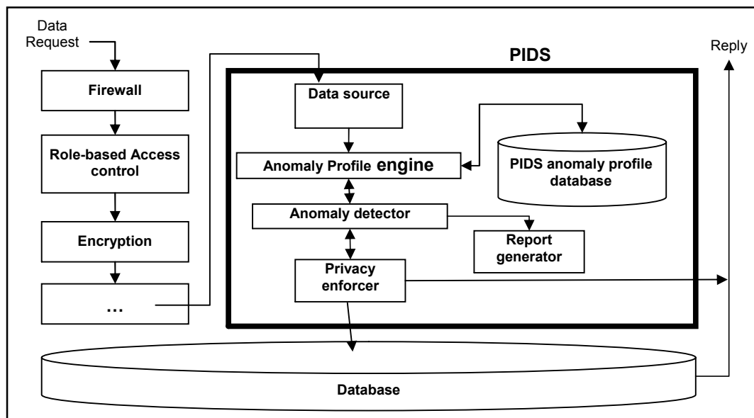
Figure 1: Model for a privacy IDS
